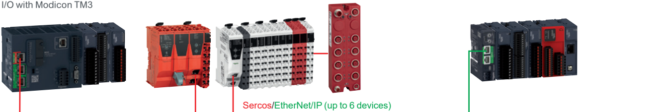
Modicon TM5 Safety logic controller, Modicon TM5 Sercos interface module, Modicon TM5 Safety I/O, Modicon TM7 Safety I/O
